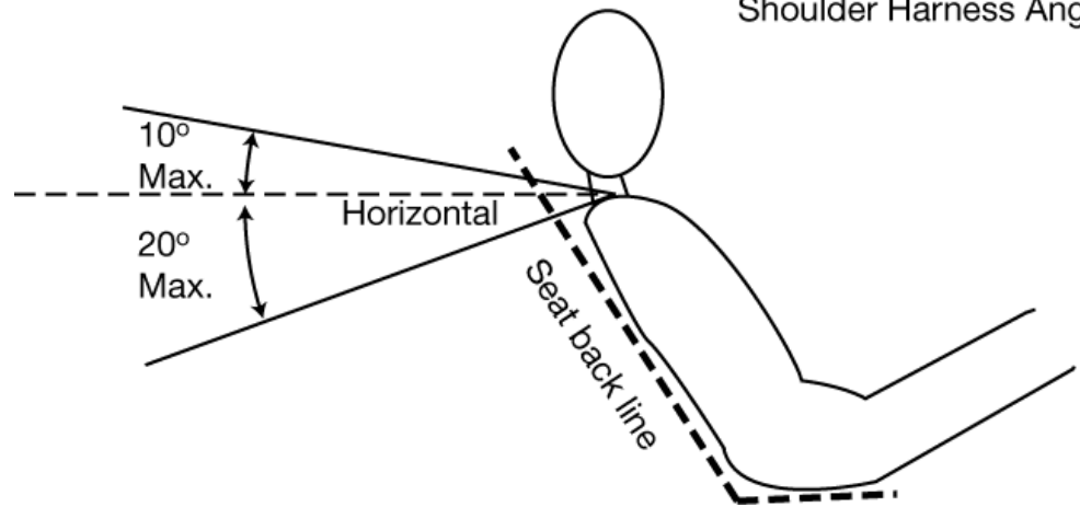
FIGURE 6 b Shoulder Harness Angle
