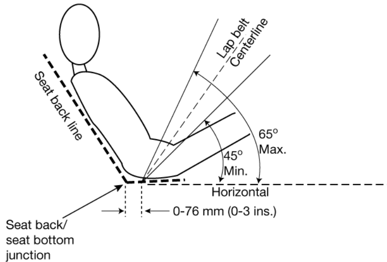
FIGURE 6 a Lap Belt Angle
